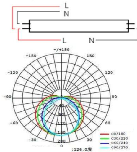
Single/Double end input option
